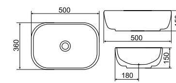
MODUO 50 SQUARE / CERSANIT
