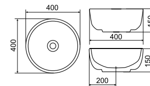
MODUO 40 RING / CERSANIT
